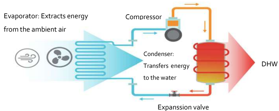
Figure 1: Operating principle
